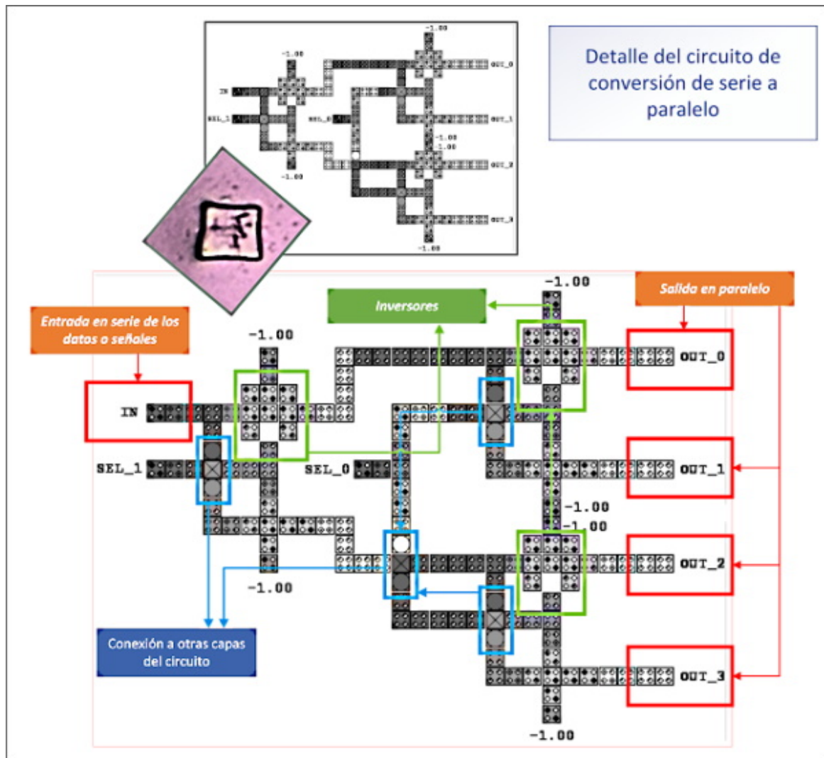
Fig. 7. Details of the circuit for converting TS-00K signals in series to a parallel output, confirming one of the typical tasks of a router. (Sardinha, L.H .; Costa, A.M .; Neto, O.P.V .; Vieira, L.F .; Vieira, M.A. 2013)
