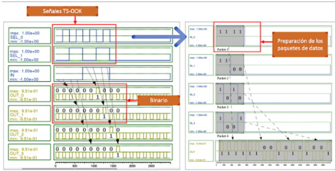
Fig. 8. The tests of the demux circuit, already observed in figure 7, provide the proof of how the TS-00K signals are interpreted and converted to the binary code, to finally generate the data packets of the corresponding nanocommunications protocol. (Sardinha, L.H .; Costa, A.M .; Neto, O.P.V .; Vieira, L.F .; Vieira, M.A. 2013)
